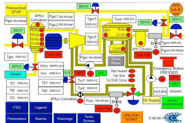
Fig. 7 – Programming design of the technological diagram screen for a screw electro-compressor.
