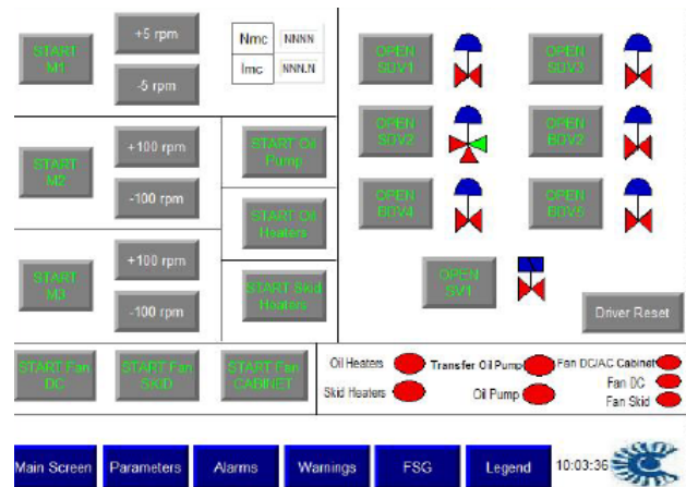
Fig. 11 – Programming design of the compressor test screen.
