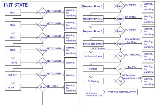
Fig. 2 – Init state logic diagram for PLC software.
