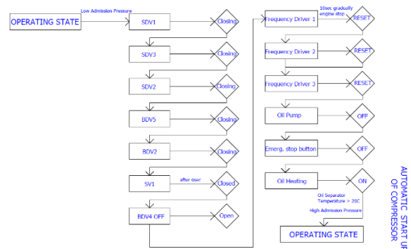
Fig. 6 – Stand-by state logic diagram for PLC software.
