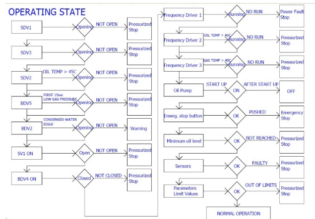
Fig. 3 – Operating state logic diagram for PLC software.
