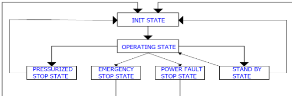
Fig. 1 - Programmable logic controller software states of a screw compressor.
