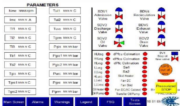
Fig. 8 – Programming design of the parameter screen for a screw electro-compressor.
