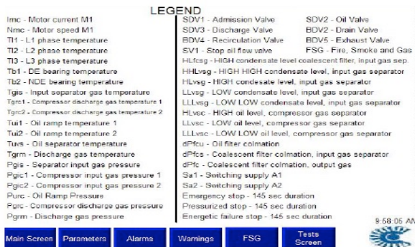
Fig. 9 - Programming design of the legend screen for a screw electro-compressor.
