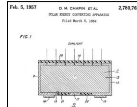
Fig. 2 – Patent of the first practical silicon solar cell [4].
