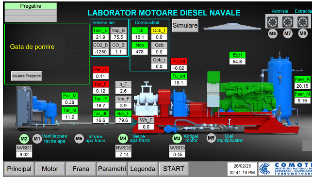
Fig. 11 – The technological diagram screen, in Preparation phase.
