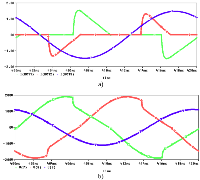
Fig. 4 – a) the waveforms of the currents corresponding to the three phases of the distorting consumer 1; b) the waveforms of the voltages at the terminals of the distorting consumer 1.
