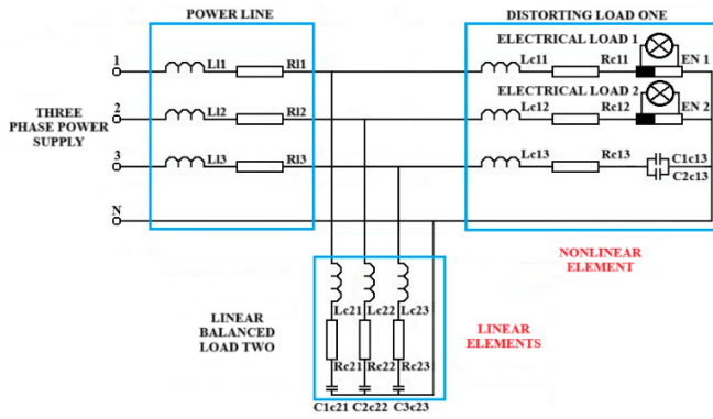
Fig. 1 – Detailed description of the experimental electrical circuit.
