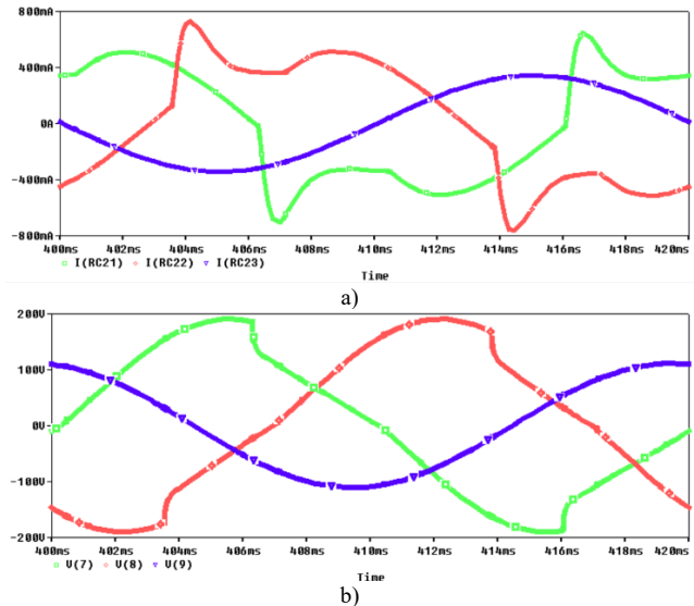
Fig. 5 – a) the waveforms of the currents corresponding to the three phases of the balanced consumer 2; b) the waveforms of the voltages at the terminals of the balanced consumer 2.
