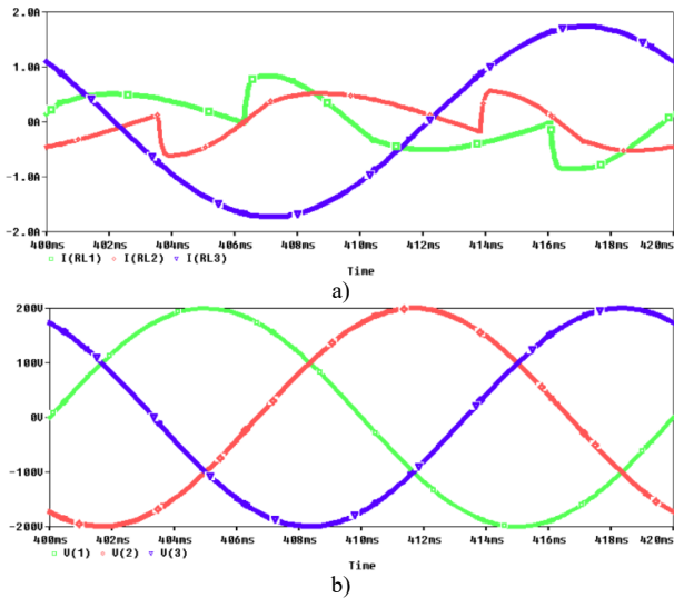
Fig. 3 – a) the waveforms of the three-phase system of currents corresponding to the three phases of the supply line; b) the waveforms of the three-phase, symmetrical supply voltage system of direct succession.
