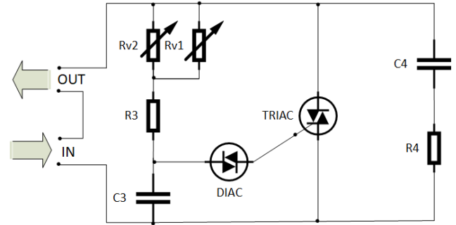
Fig. 2 – Detailed description of identical circuits EN_1 and EN_2 .
