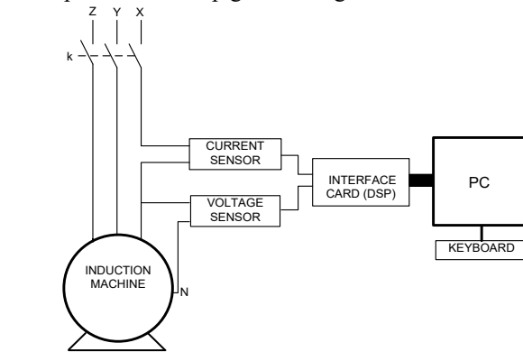
Fig. 6 – Measurement setup.
