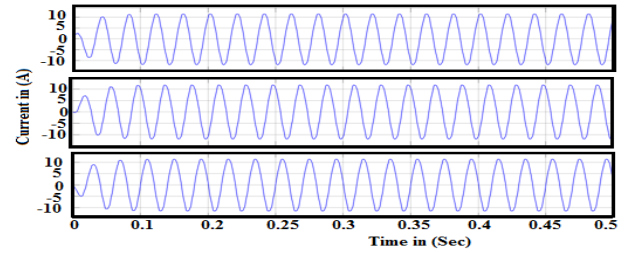
Fig. 11 – Inverter output current waveform.
