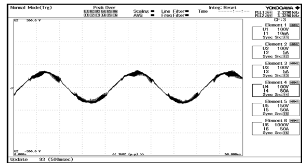
Fig. 19 – Trans QZSI output voltage waveform after LC filtering.
