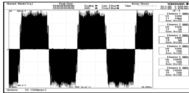
Fig. 18 – Trans quasi-Z-source inverter output voltage waveform before LC filtering.
