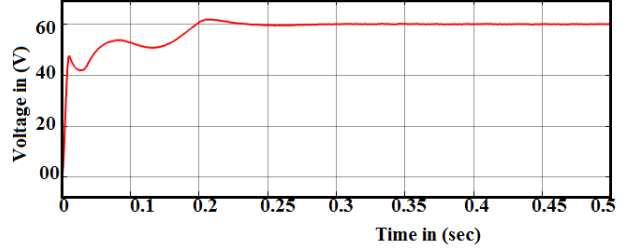
Fig. 9 – Z-source network output.
