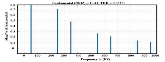
Fig. 12 – Total harmonic distortion.
