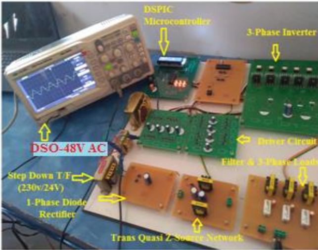
Fig. 14 – Hardware snapshot.
