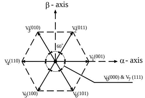
Fig. 5 – Vector diagram.
