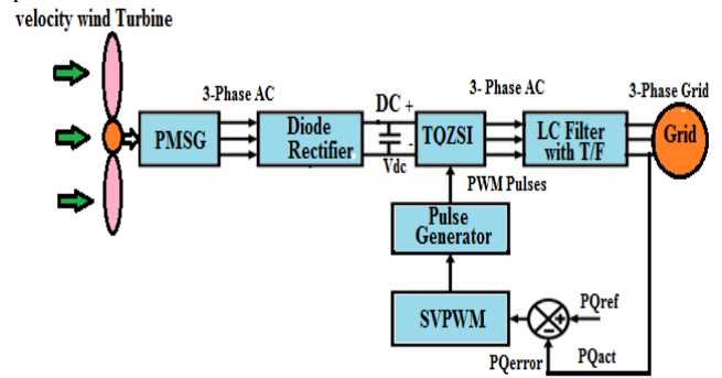
Fig. 1 – Proposed simulation block diagram.
