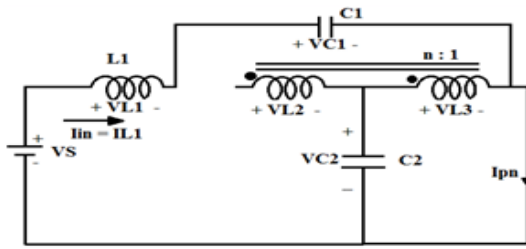
Fig .3 - Shoot through mode.
