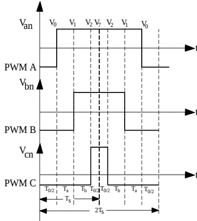
Fig. 6 – Switching state sector I.
