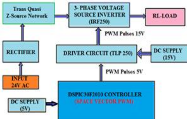
Fig. 13 – Hardware block diagram of proposed system.
