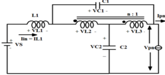
Fig. 4 – Non-shoot-through mode.
