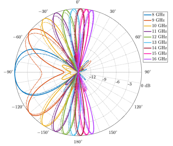
Fig. 4 – Simulated (solid) and measured (dashed) LHCP radiation pattern of the manufactured prototype at different frequencies in the xz-plane.
